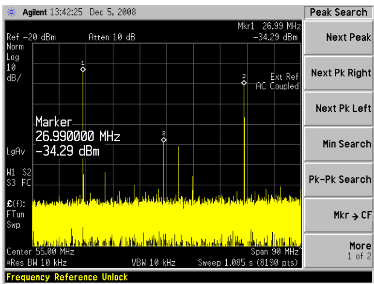
FIGURE 9 - Spectrum Analyzer Measurement of XTAL OUT Output of Channel 8, AC Coupled, 1K \Omega Terminations
