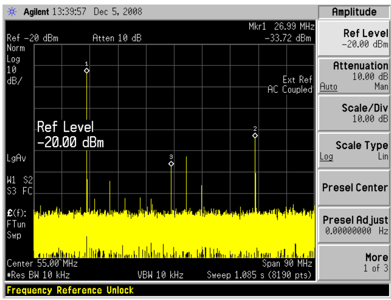
FIGURE 8 - Spectrum Analyzer Measurement of XTAL OUT Output of Channel 1, AC Coupled, 1K \Omega Terminations
