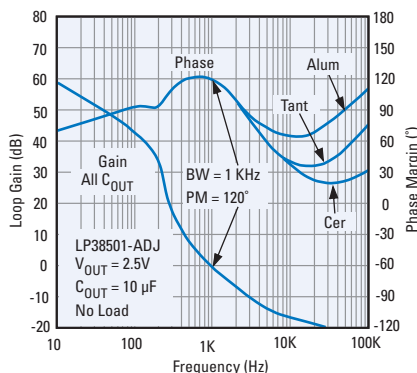
Figure 3. Gain/Phase Plot for No Load Operation with Various C_{OUT} Types
