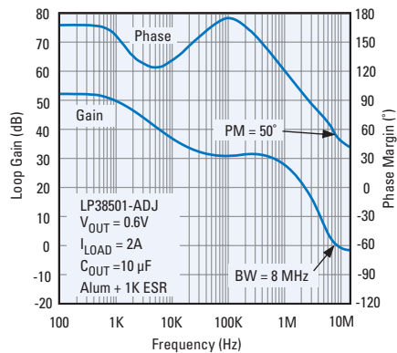
Figure 4. Gain/Phase Plot for Aluminum Output Capacitor with 1K ESR
