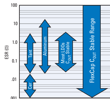
Figure 1. ESR Ranges for Various Output Capacitor Types
