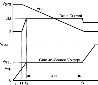
a) Current Limit Only
