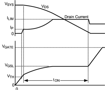
b) Power Limit and Current Limit
