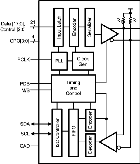
DS92LX2121 - SERIALIZER
