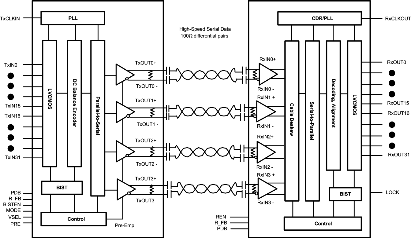
Tx - SERIALIZER
