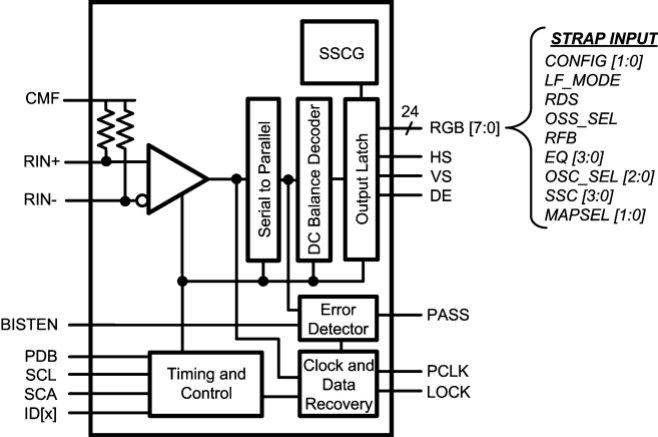
DS90UR906Q – DESERIALIZER
