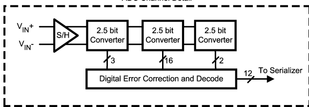
ADC Channel Detail
