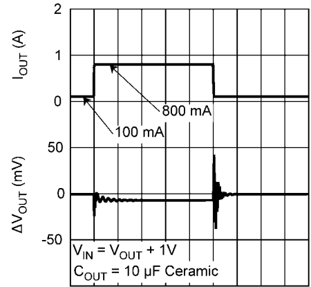
Load Transient Response, C_{OUT} = 10 \mu\text{F} Ceramic
