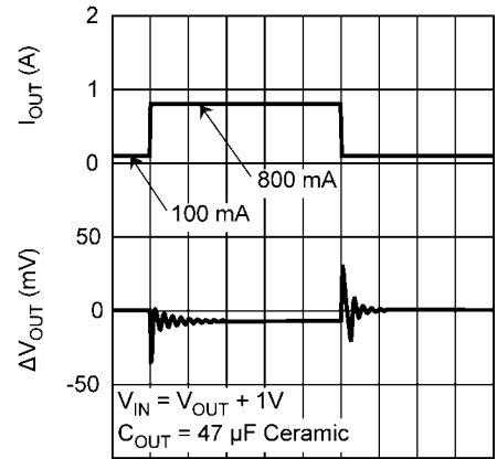
Load Transient Response, C_{OUT} = 47 \mu\text{F} Ceramic
