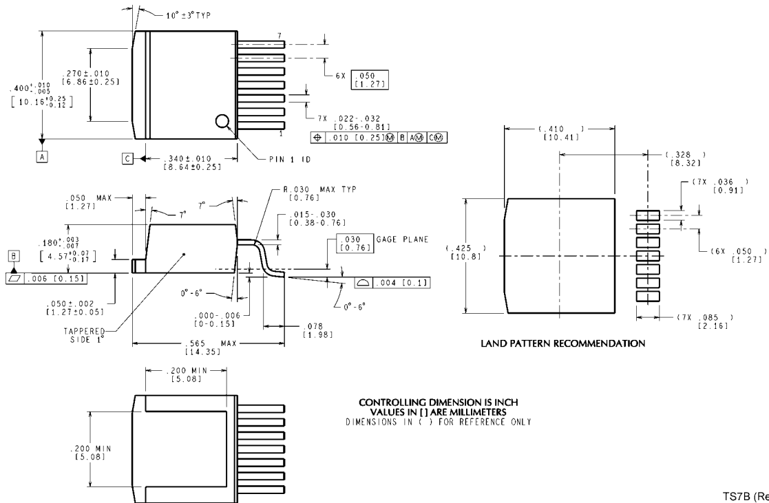
CONTROLLING DIMENSION IS INCH VALUES IN [ ] ARE MILLIMETERS DIMENSIONS IN ( ) FOR REFERENCE ONLY TO-263 7-Lead, Molded, Surface Mount Package (TO263-7) NS Package Number TS7B
