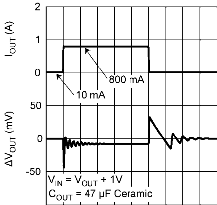
Load Transient Response, C_{OUT} = 47 \mu\text{F} Ceramic
