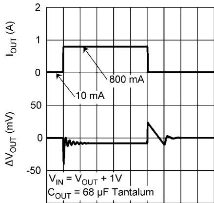
Load Transient Response, C_{OUT} = 68 \mu\text{F} Tantalum
