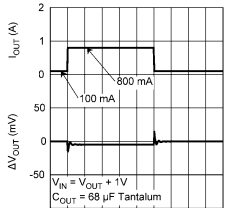
Load Transient Response, C_{OUT} = 68 \mu\text{F} Tantalum
