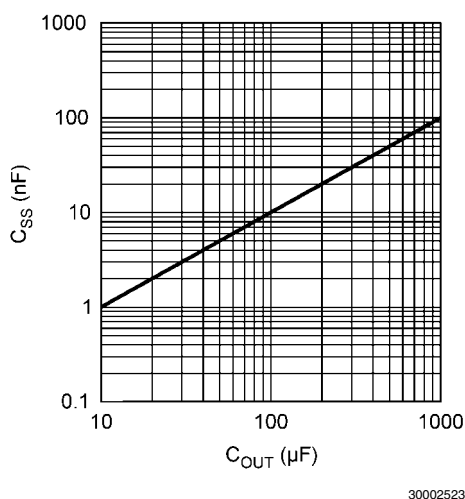
FIGURE 2. Typical C_{SS} vs C_{OUT} Values
