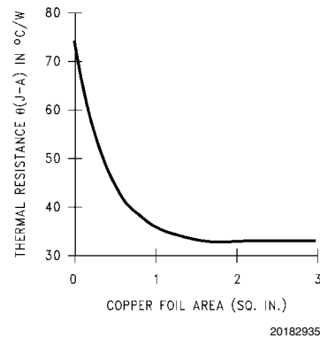
FIGURE 3. θ JA vs Copper (1 Ounce) Area for TO-263 package
