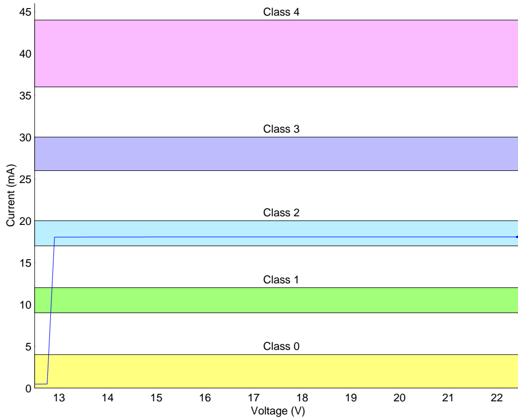
Figure 4: Mode B Classification Signature Characteristics – Class 2
