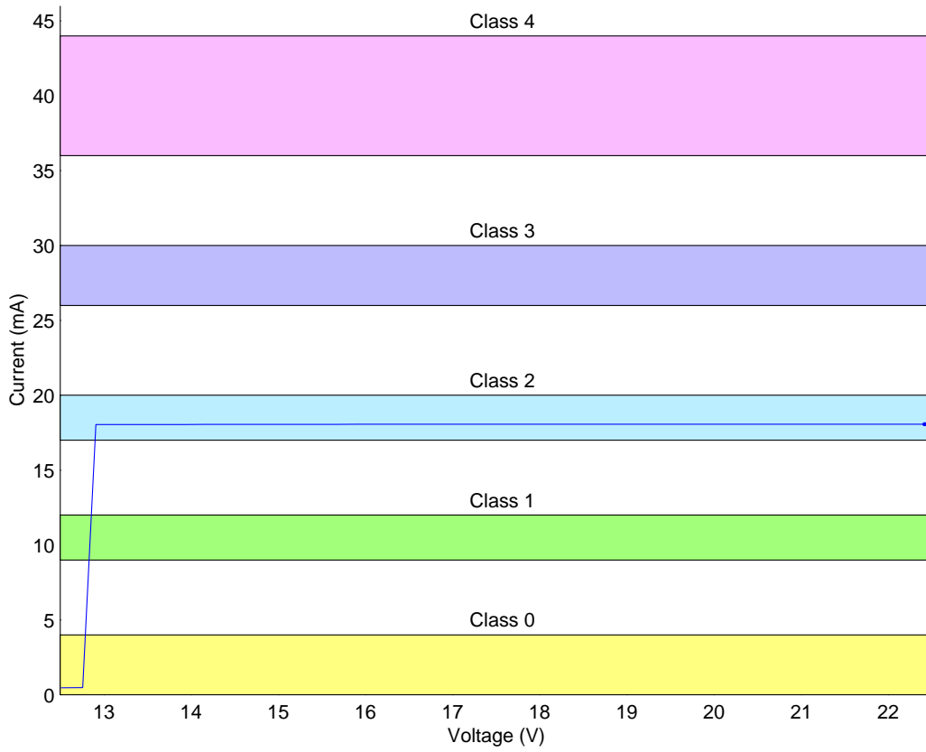
Figure 3: Mode A Classification Signature Characteristics – Class 2
