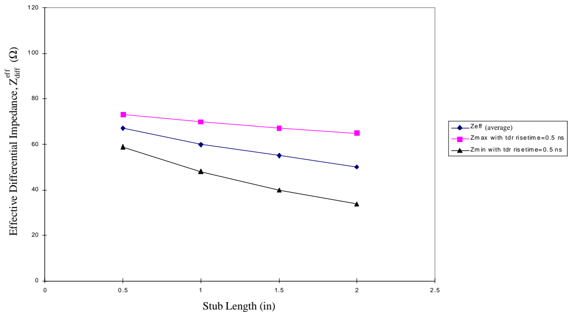
Figure 4. – Differential Impedance (min, max and effective) vs. Stub Length For PCB raw etch Z_{diff} = 100 \Omega and TDR rise time = 0.5ns.
