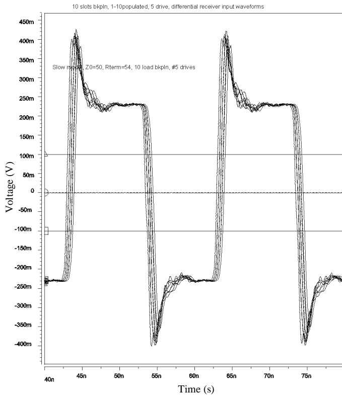
Figure B6 (left) shows similar data for the 10-slot backplane configuration but, with the card in slot 5 driving the bus. The differential waveforms shown are at the inputs to the receivers at slots 1-4 and 6-10.
