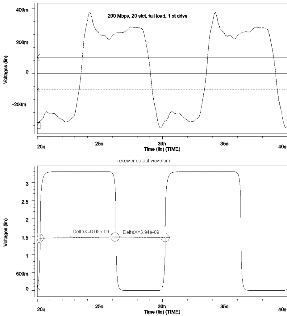
Figure C2 – Receiver input (above) and output; high/low bit sequence running at 200 Mbps.
