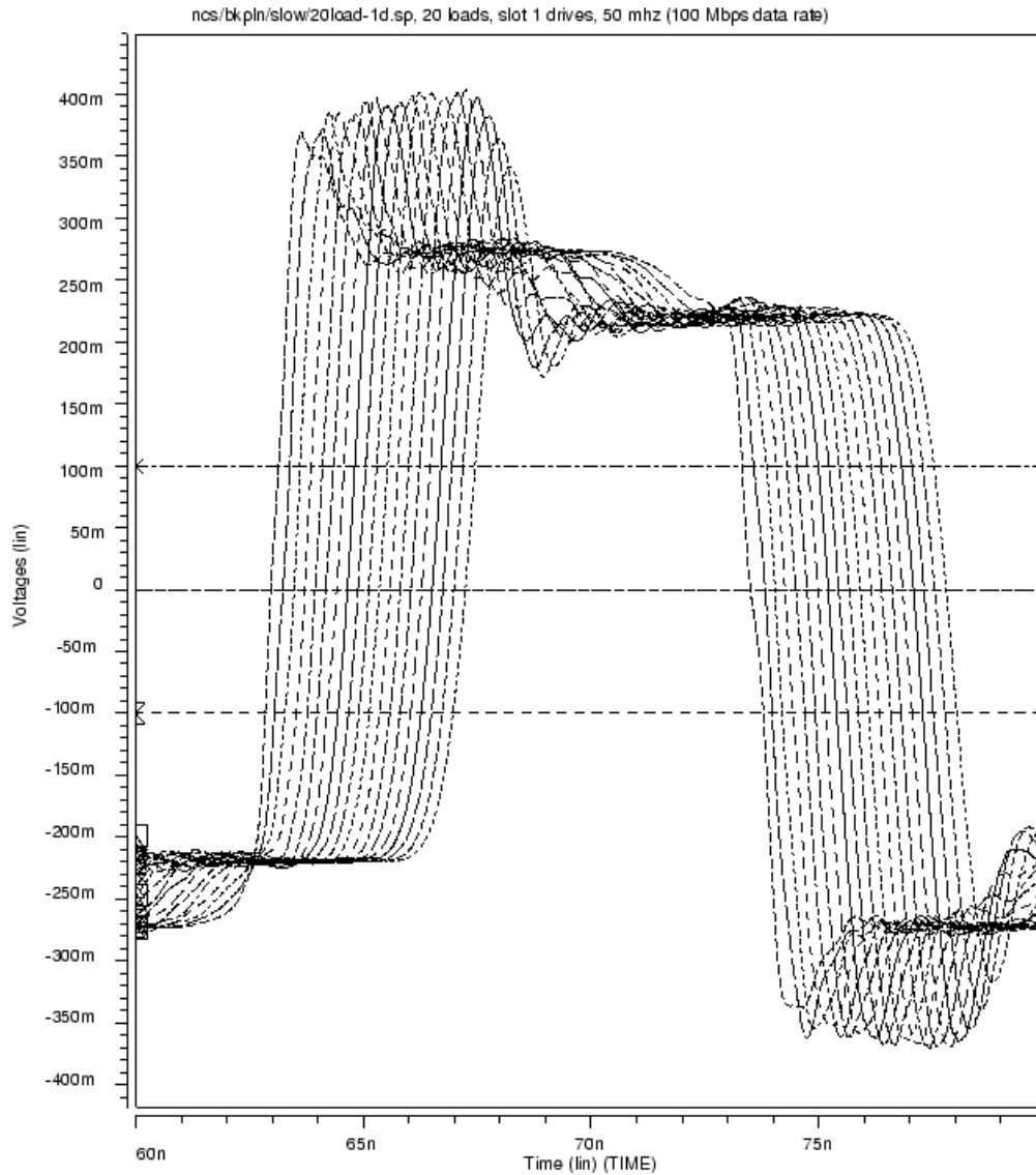
Figure 2 – 20-slot BLVDS backplane simulation results (receiver input waveforms).
