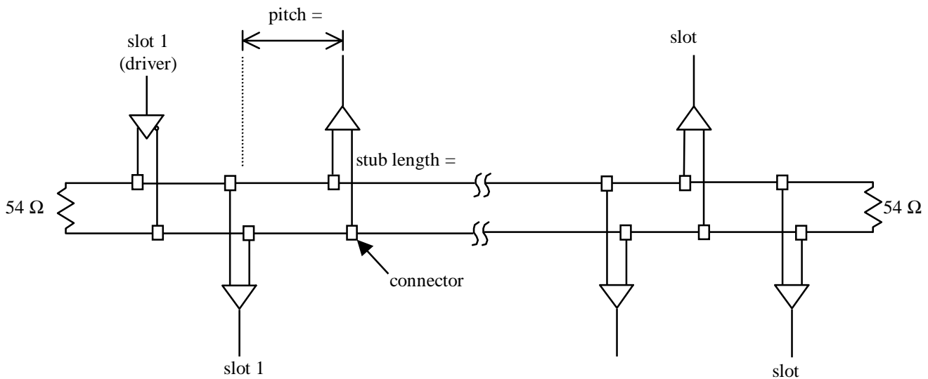
Figure 1. - The National BLVDS backplane; Z_0 = 50 \text{ Ohms (SE)} , termination resistor = 54 Ohms at each end.
