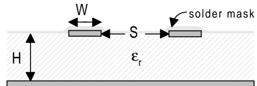
Figure 8 – Simple microstrip differential pair geometry.
