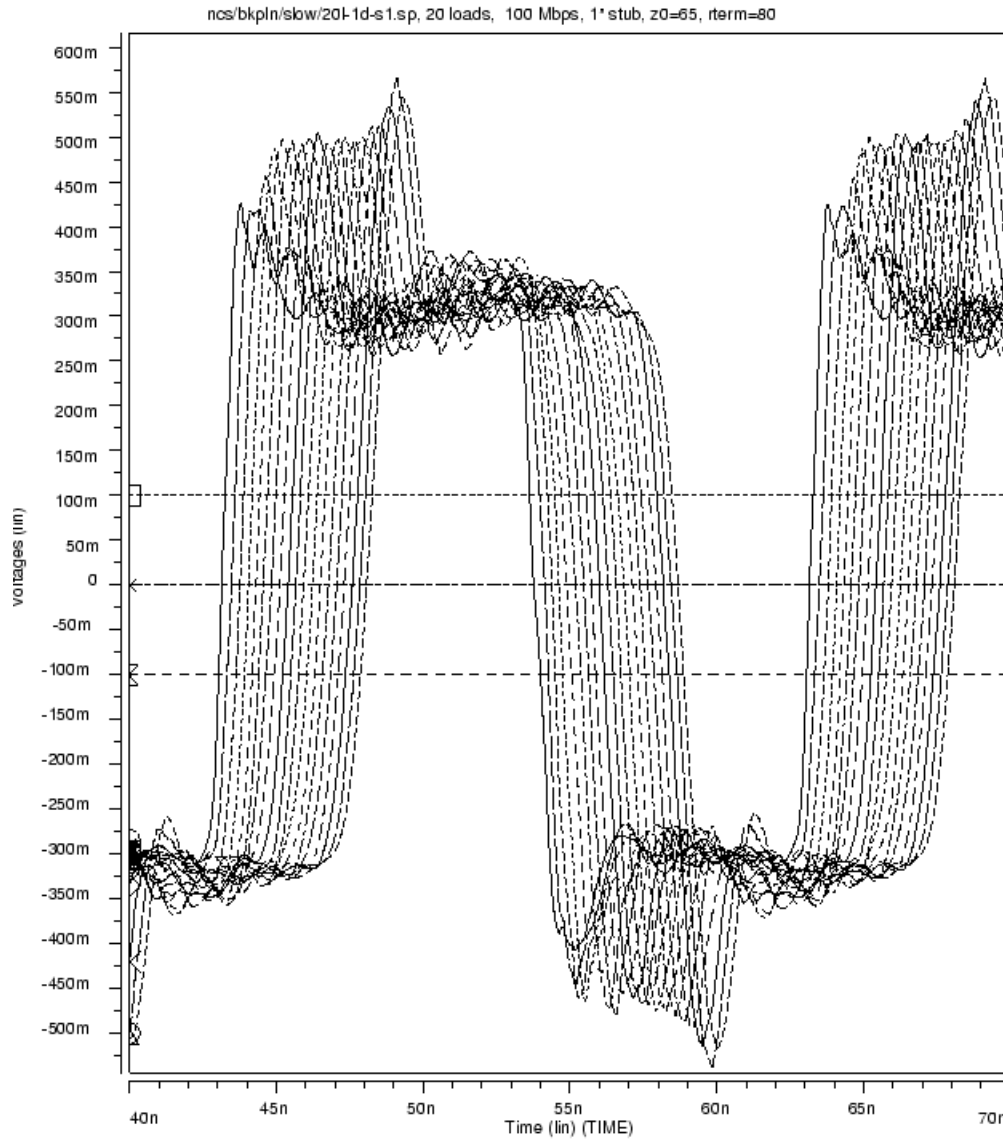
Figure 9. – BLVDS receiver input waveforms under “optimized parameter” conditions.
