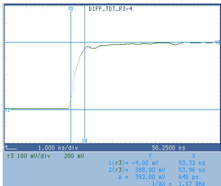
Figure A6 – TDT transmitted waveform (4-slot bus).
