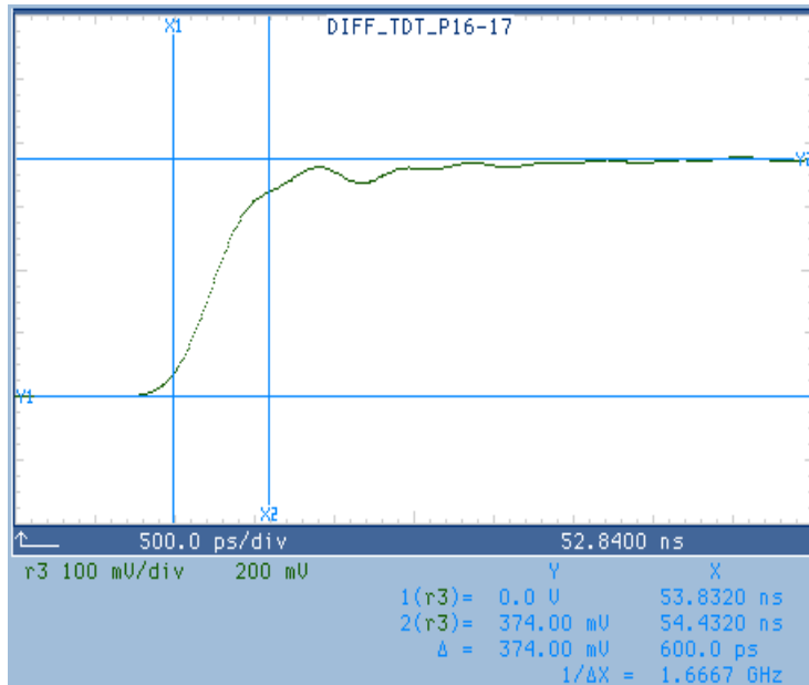
Figure A5 – TDT transmitted waveform (20-slot bus).
