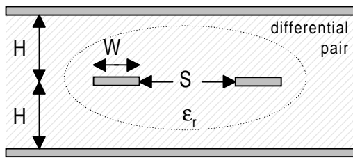
Figure 7 – Simple stripline differential pair geometry.
