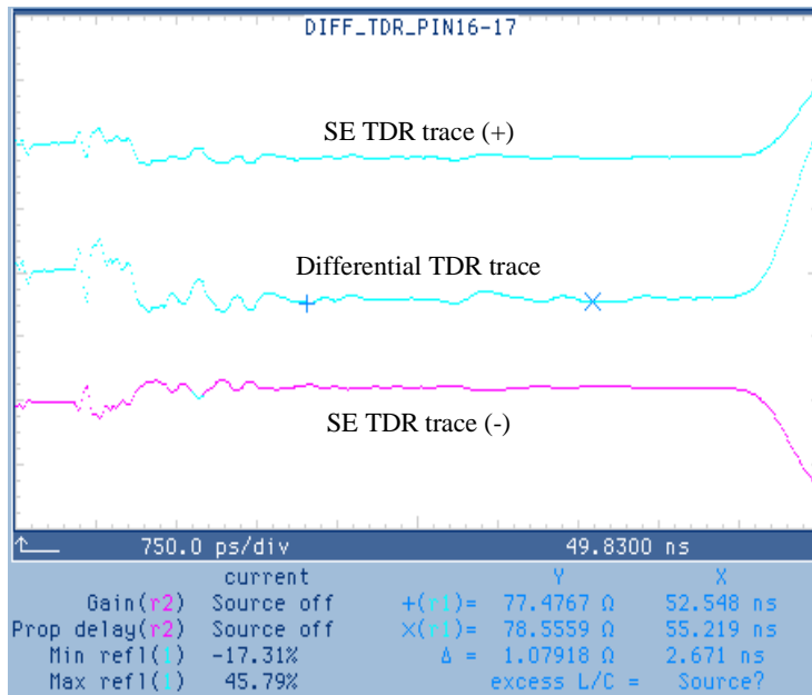
Figure A1 - Differential TDR measurement, 20-slot backplane.
