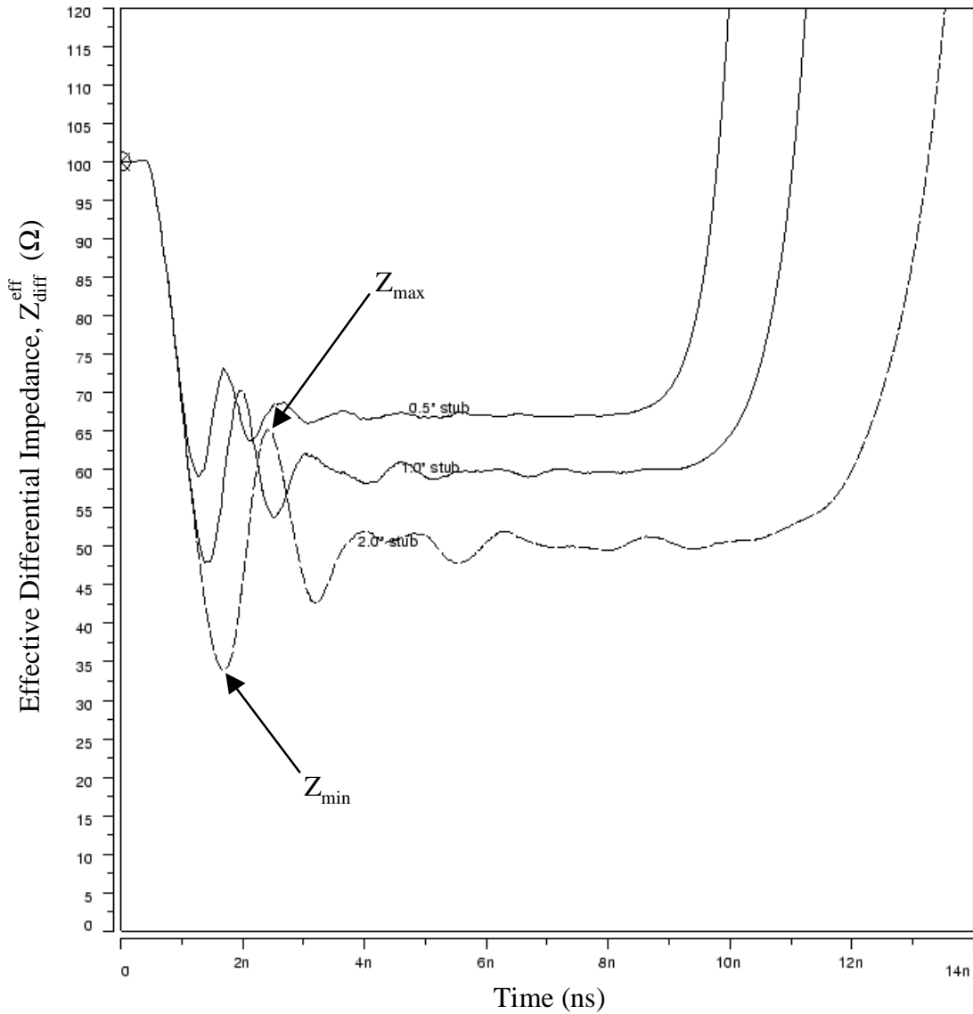
Figure 3. - TDR simulation for a fully loaded 20-slot BLVDS backplane, TDR rise time = 0.5 ns, PCB differential etch impedance = 100 \Omega
