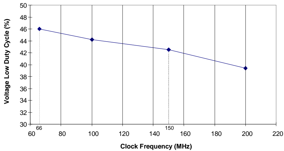
Figure C3 – Low data bit duty cycle vs. clock frequency.
