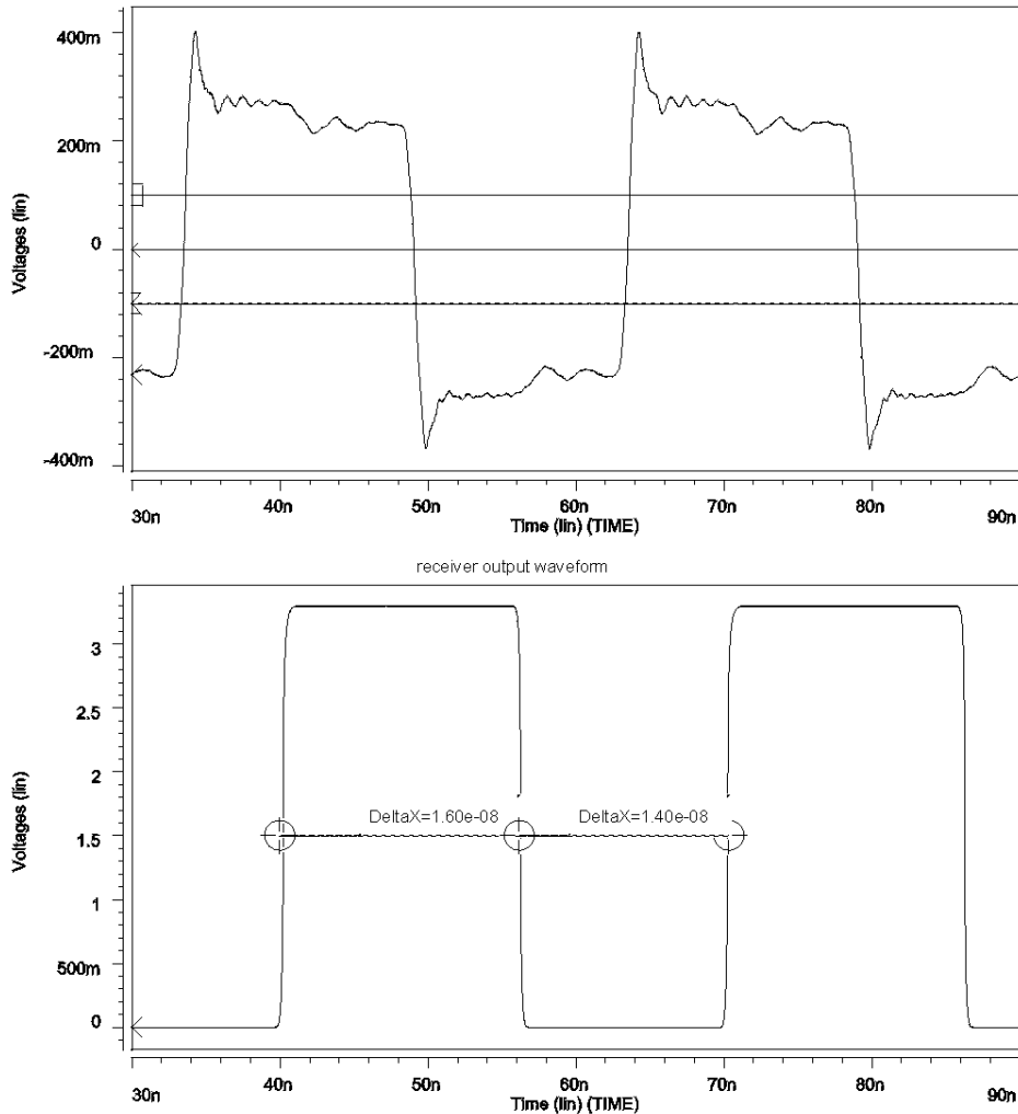
Figure C1 – Receiver input (above) and output; high/low bit sequence running at 66 Mbps.
