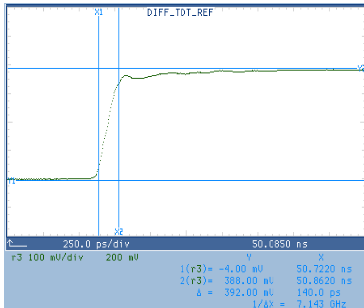
Figure A4 – TDT reference (incident) waveform.
