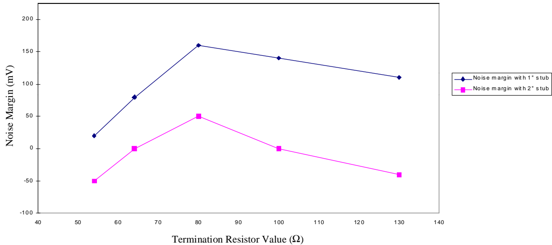
Figure 6. - Noise Margin vs Termination Resistance Value for Two Stub Lengths at 100 Mbps Data Rate (active simulation).
