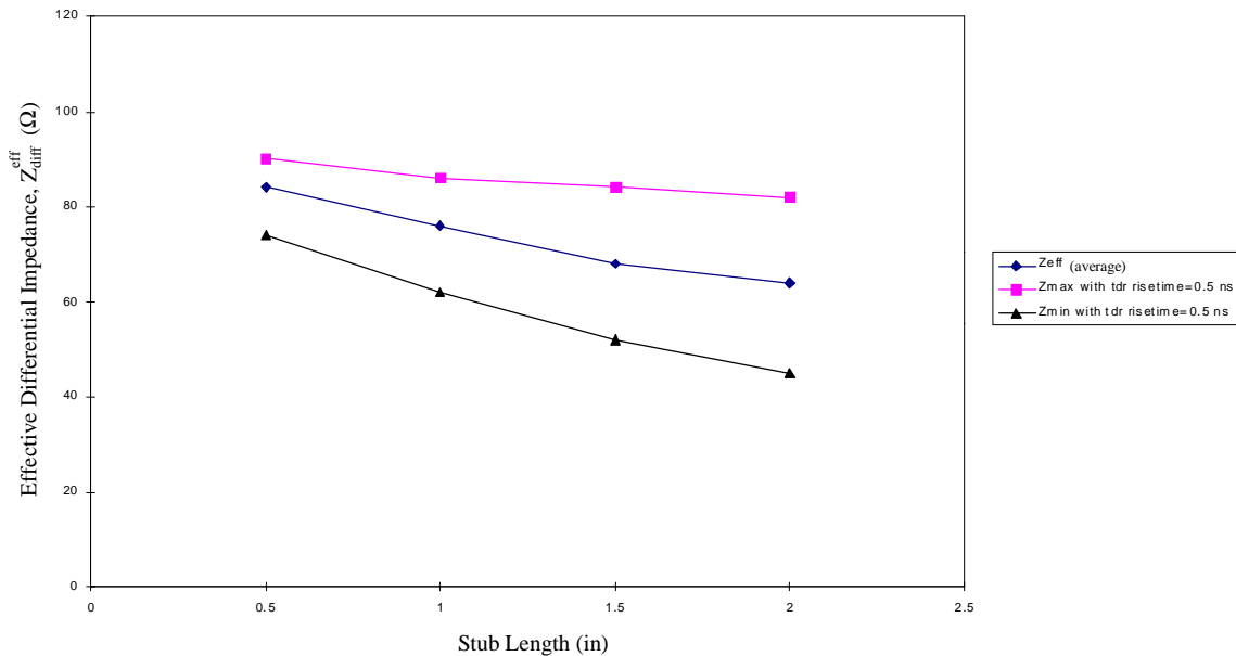
Figure 5. – Effective Diff. Impedance (min, max and average) vs. Stub Length For PCB raw etch Z_{diff} = 130 \Omega and TDR rise time = 0.5ns.
