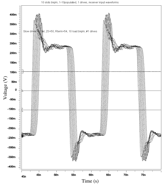
Figure B5 (right) shows the differential receiver input waveforms at slots 2-10 for a 10-slot BLVDS backplane with the card in slot 1 driving the bus.
