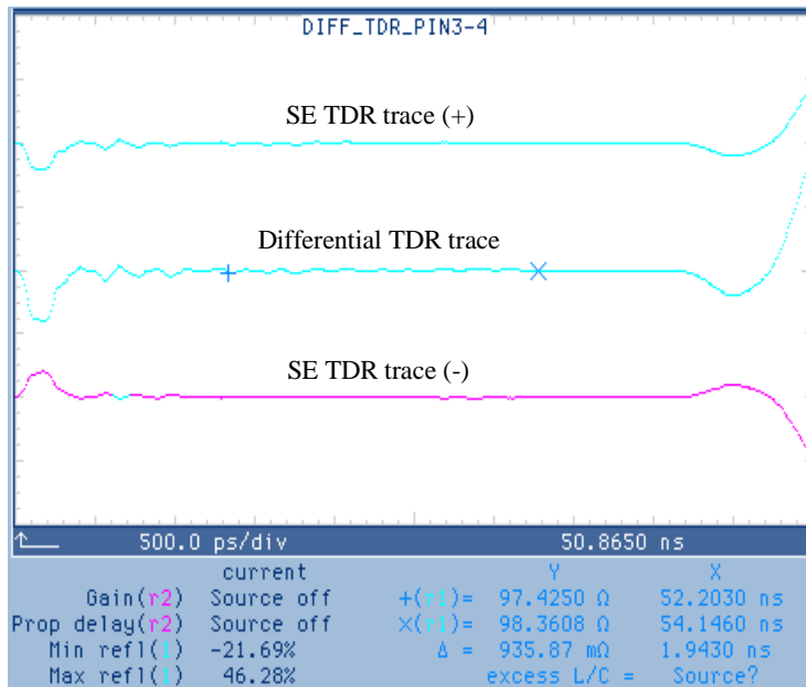
Figure A2 - Differential TDR measurement, 4-slot backplane.
