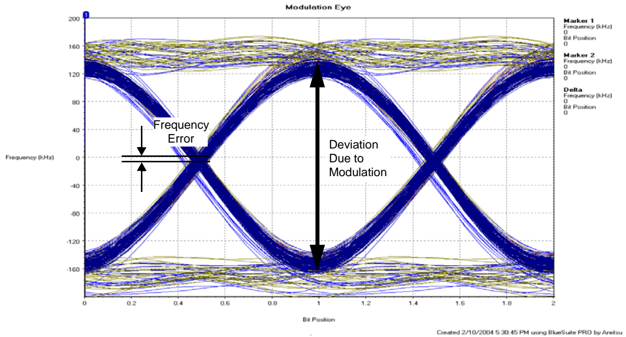
Figure 6. Eye Diagram
