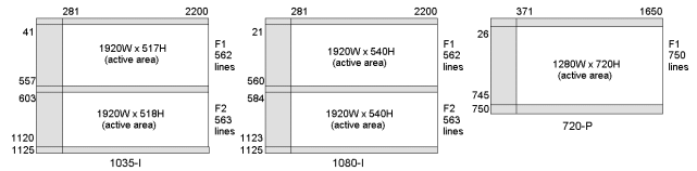
Figure 8 – Source Format Mappings
