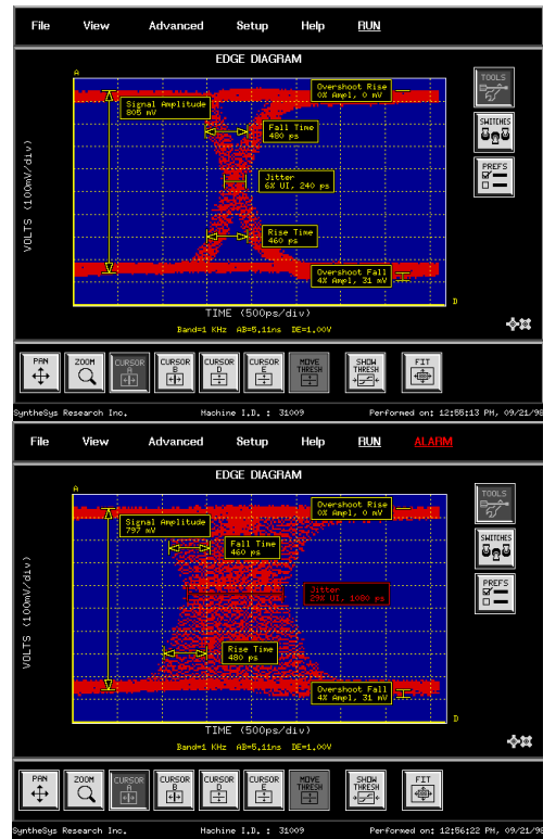
Figure 21 – Edge™ Diagrams (Example SDI signal)
