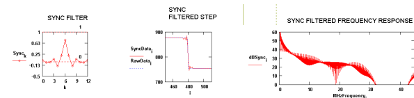
Figure 12 – Sync-Filtered Luminance Response
