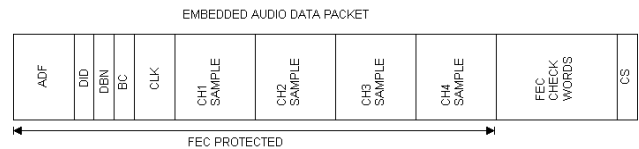
Figure 19 – Embedded Audio Data Packet
