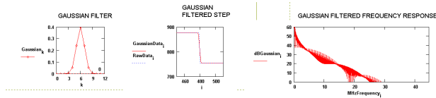
Figure 11 – Gaussian-Filtered Luminance Response
