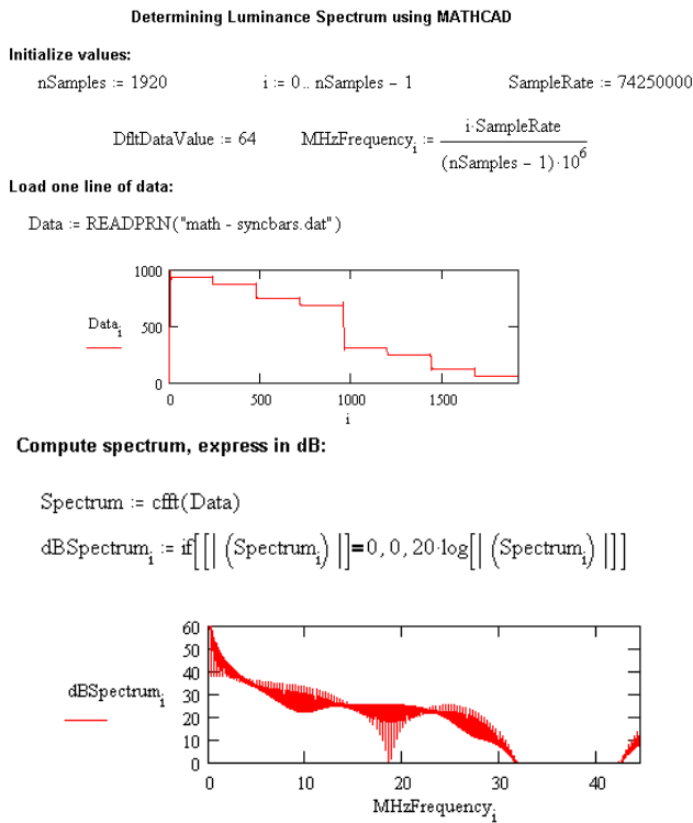
Figure 24 – FFT Worksheet in MathCAD™
