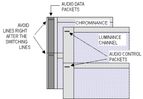
Figure 18 – Embedded Audio Mapping
