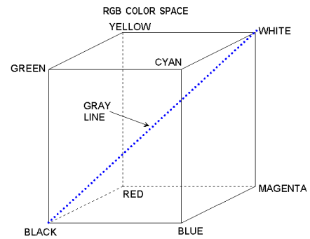
Figure 13 – RGB Colorspace
