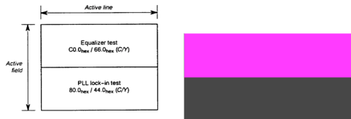
Figure 22 – Pathological Test Pattern 16
