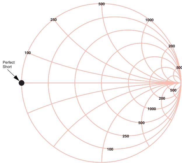
Figure 15. Smith Chart, Perfect Short
