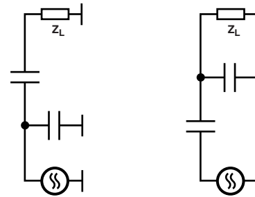
Figure 23. Two Possible Matching Networks
