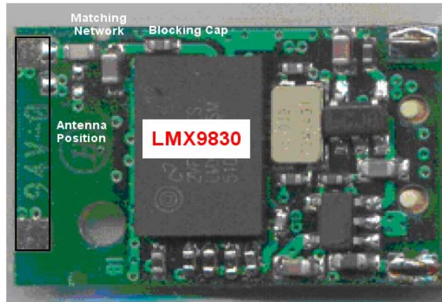
Figure 13. LMX9830 Antenna
