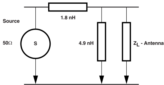
Figure 19. Impedance Matching Network
