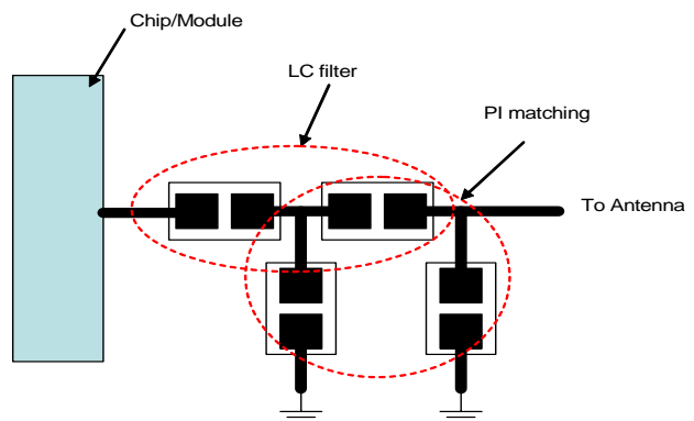
Figure 32. Front-end layout using T PI pad
