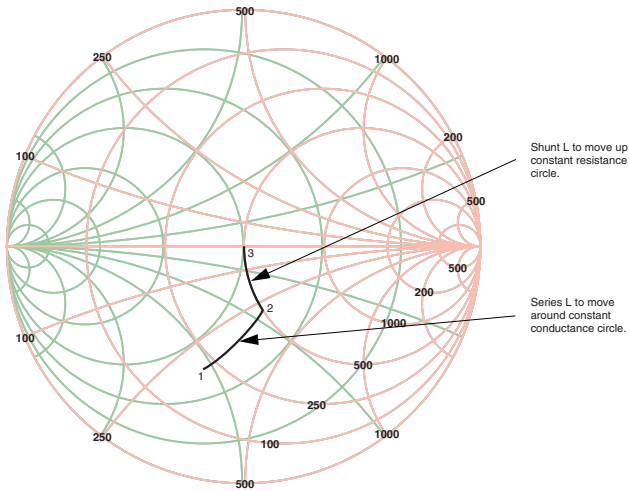
Figure 18. Impedance Transformation
