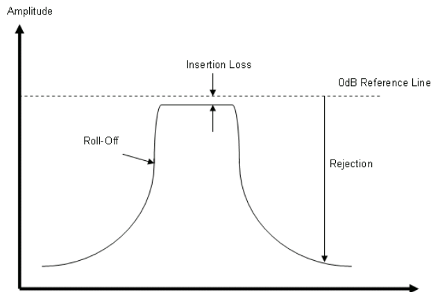
Figure 29. RF Filter Performance
