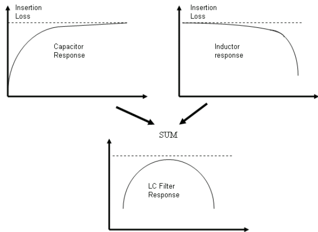
Figure 30. LC Filter Response
