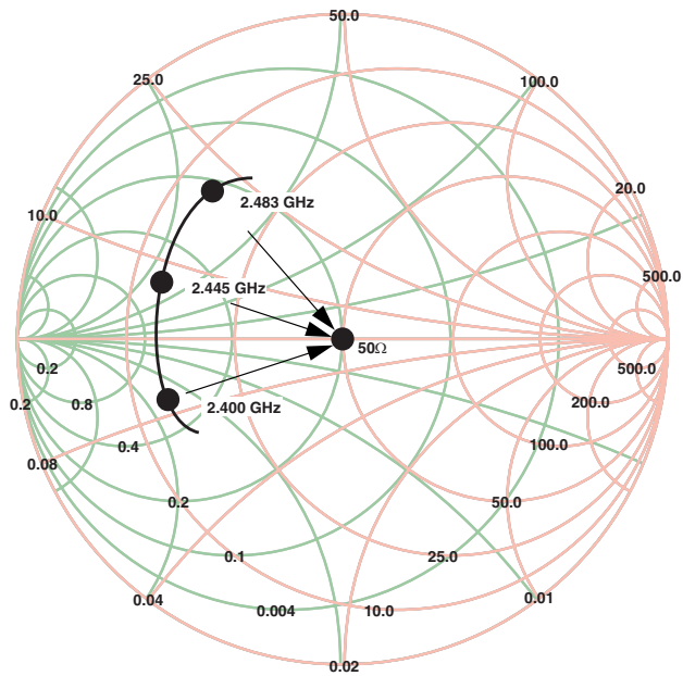
Figure 24. Broadband Match
