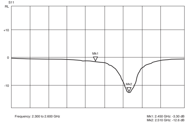
Figure 16. Return Loss, Antenna Connected
