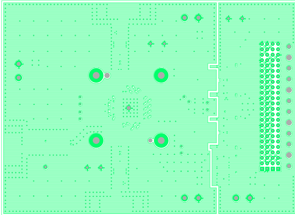
Layer 2: Ground
