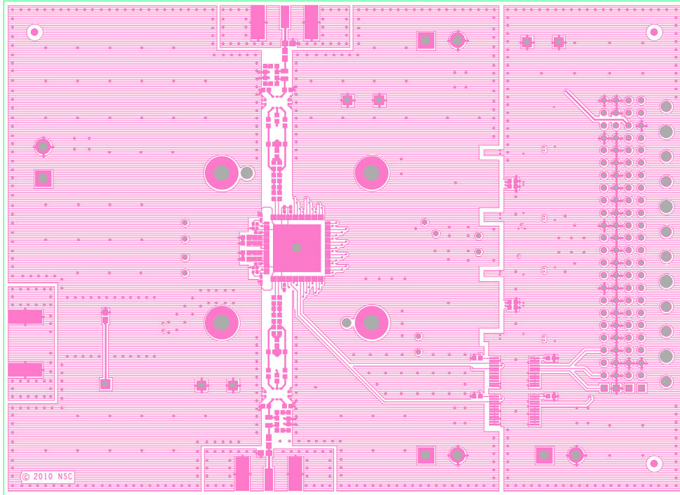
Layer 1: Component Side
