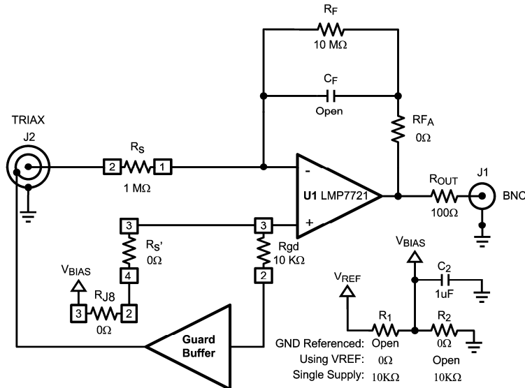
Figure 3. Simplified Inverting Schematic
