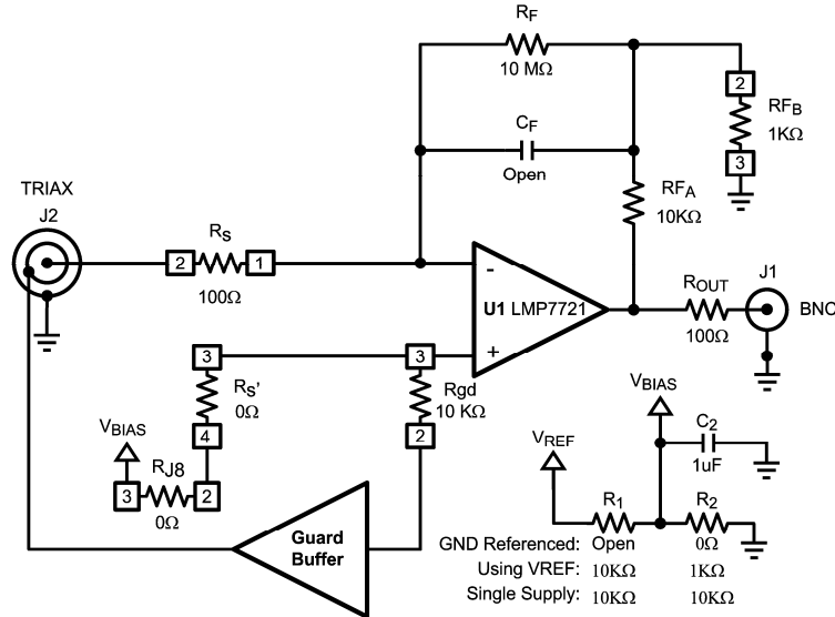
Figure 5. Simplified Transimpedance with "Tee" Feedback
