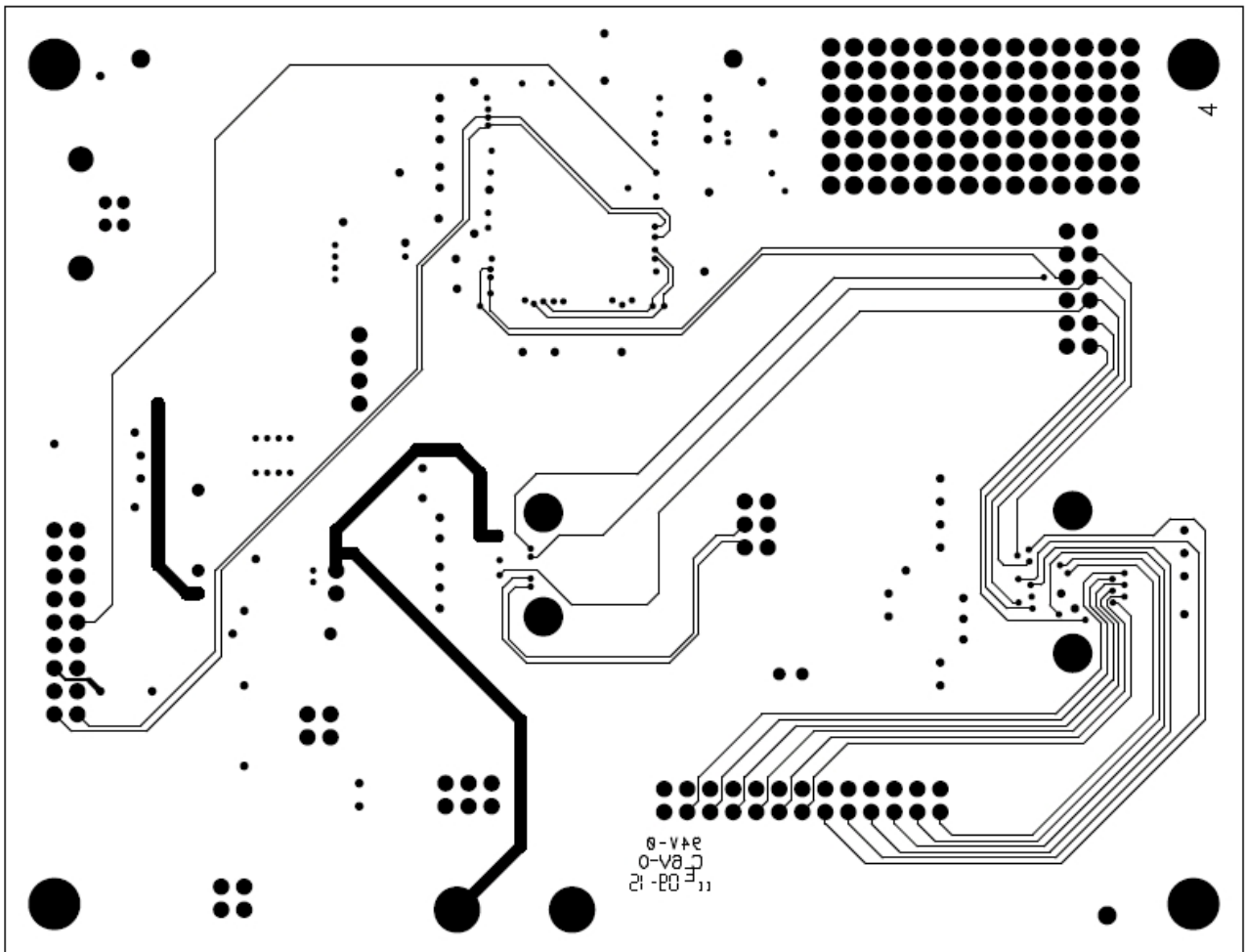
Figure 10 – Bottom Layer of the LM96080 Evaluation Board
