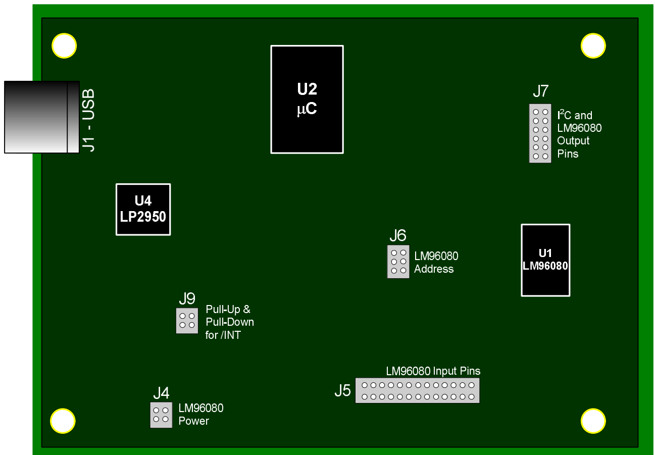
Figure 2 – Components Placement Diagram
