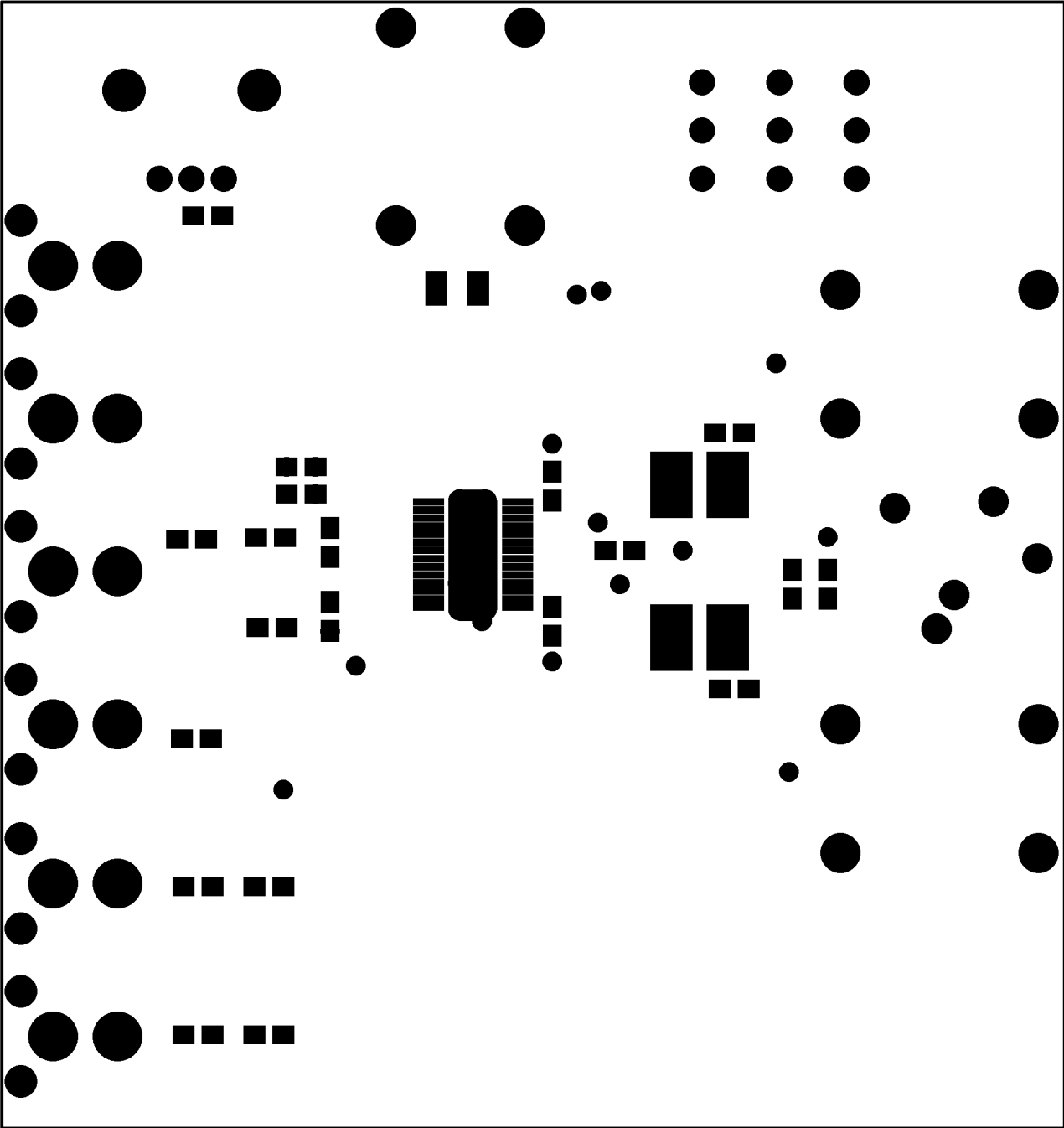
SOLDERMASK TOP
