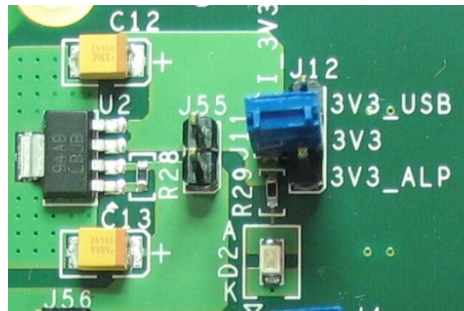
Figure 1. Default Power Supply Connection
