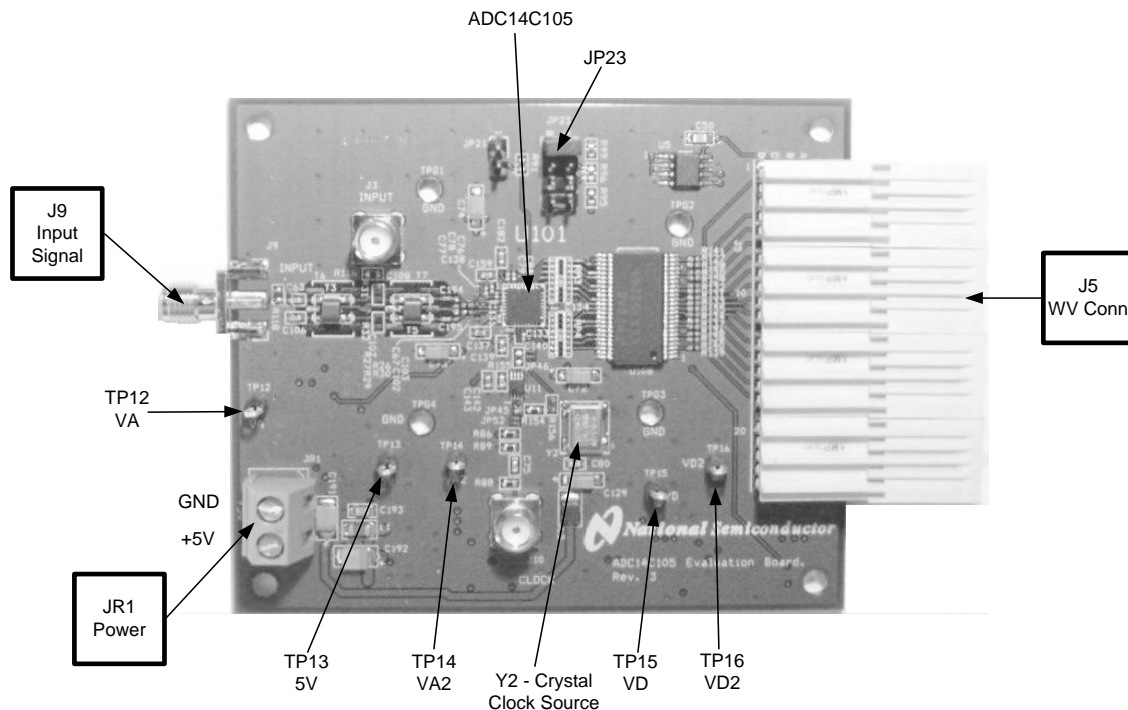
Figure 1. Major Component and Jumper Locations
