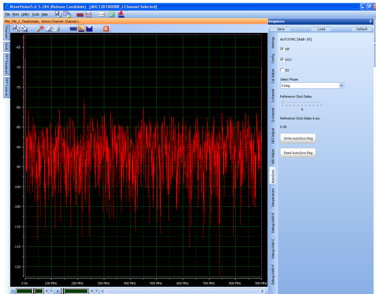
Figure 15: AutoSync Panel
