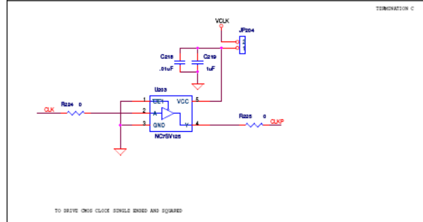
TO DRIVE CLOCK (EITHER SOURCE) SINGLE ENDED WITHOUT SQUARING
