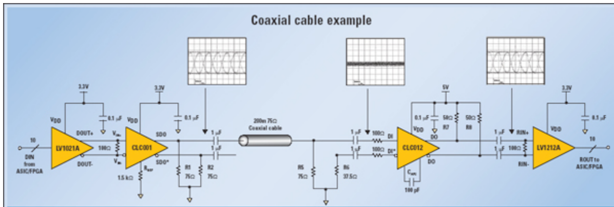
Figure 1: Example of a communication channel employing LVDS 10-bit SerDes and SDI cable driver/equalizer combo to transmit data over coaxial cable
