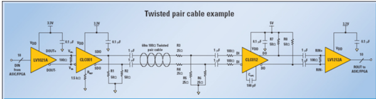
Figure 2: Example of a communication channel employing LVDS 10-bit SerDes and SDI cable driver/equalizer combo to transmit data over twisted pair cable
