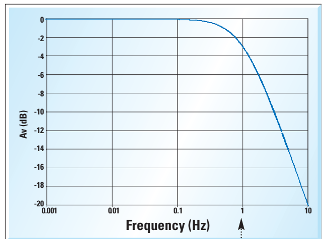
Figure 1. Normalized bandwidth curve for an op amp in unity gain (Curve assumes an open loop gain with a single pole roll-off.)
