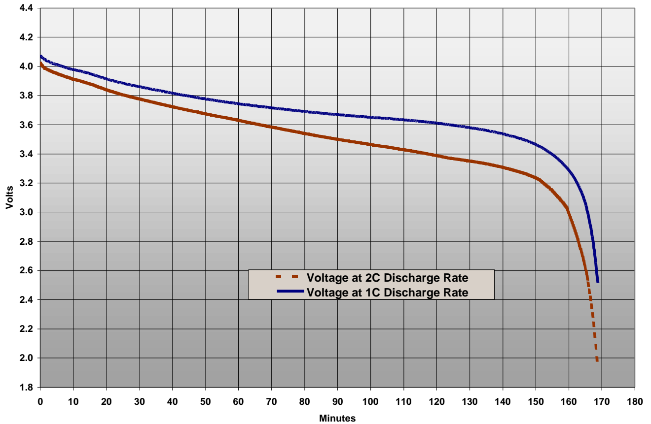
Figure 1. Although the graphite anode Lilon battery has a very flat discharge characteristic, the ESR can cause a substantial voltage drop as heavy loads are applied. 1C=275mA for this battery.
