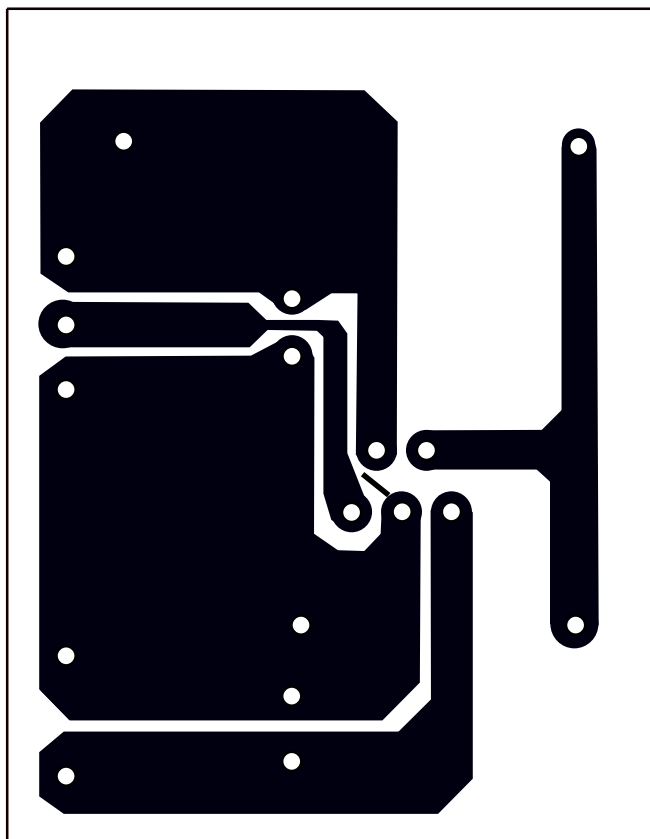
Copper side
