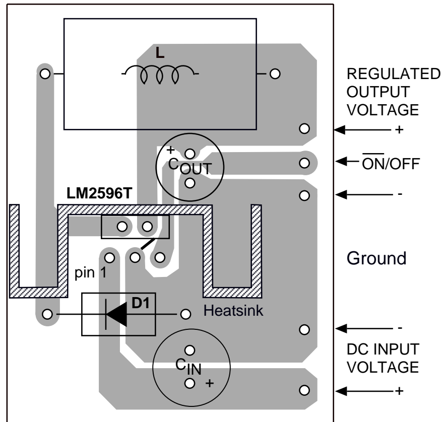
Component Side
