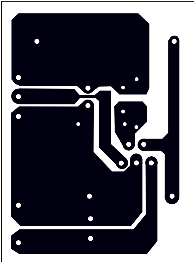
Copper side
