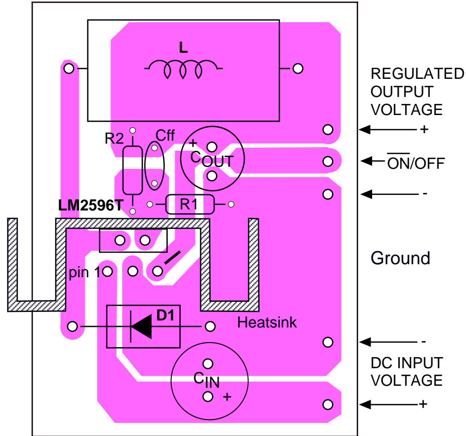
Component Side
