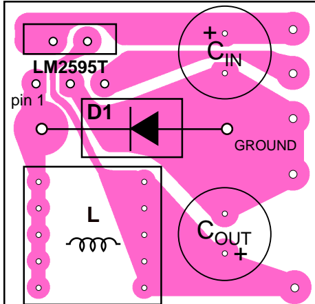
Component Side
