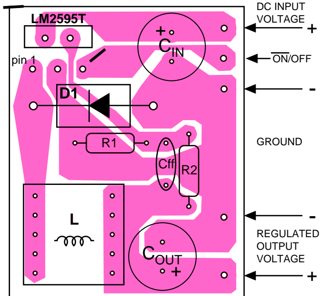
Component Side
