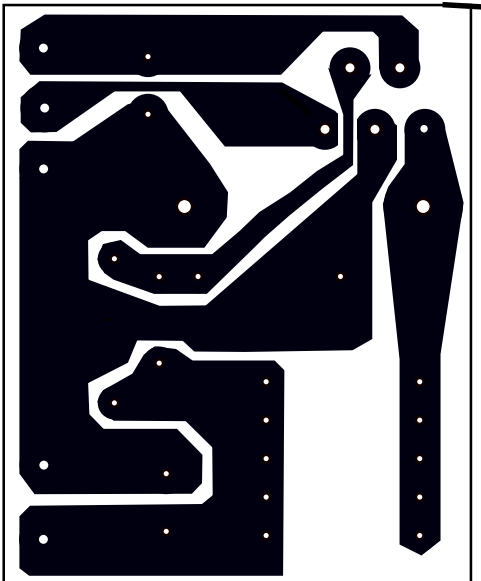
Copper side
