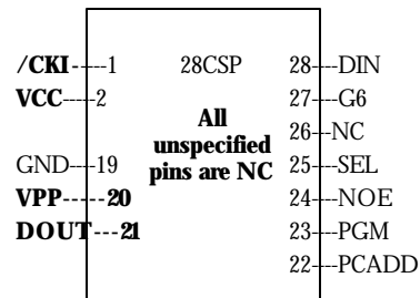
COP8Sxx7 COP8AJ/AKC7 28pin
