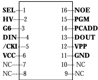
COP8Sxx7 COP8AJ/AKC7 16pin
