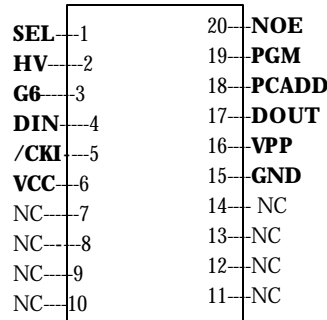
COP8Sxx7 COP8AJ/AKC7 20pin
