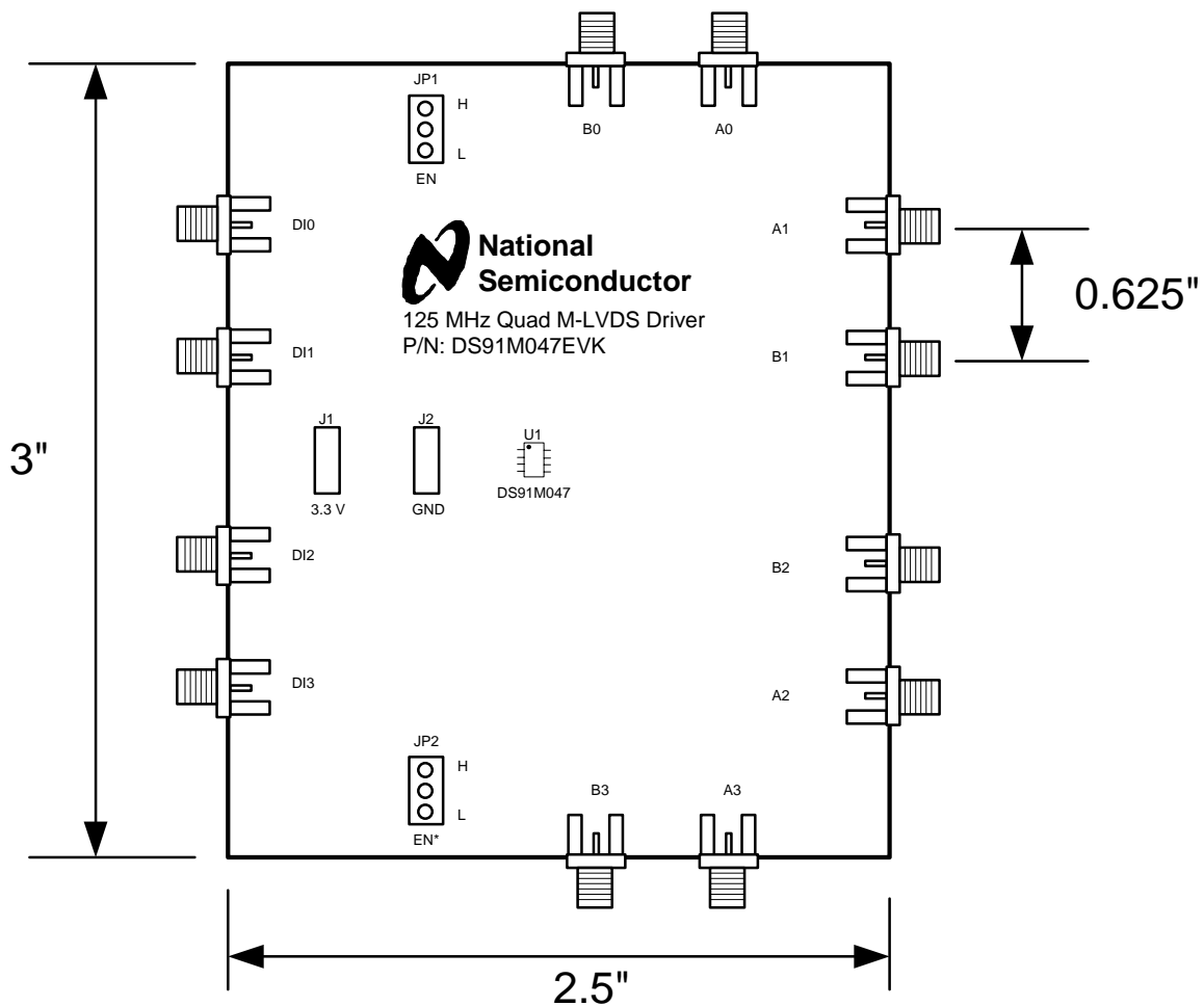
Figure 1 - DS91M047EVK Top View Drawing
