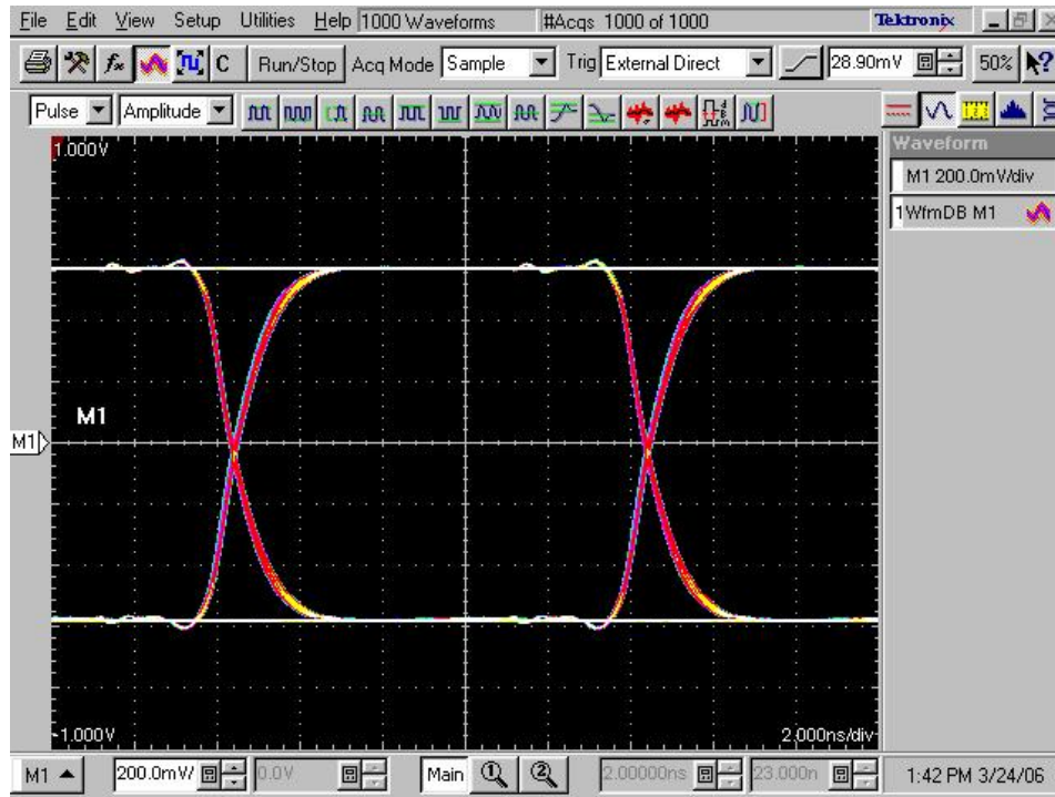
Figure 3 – DS91M047 Output
