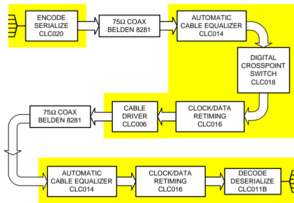
The Demonstration System
