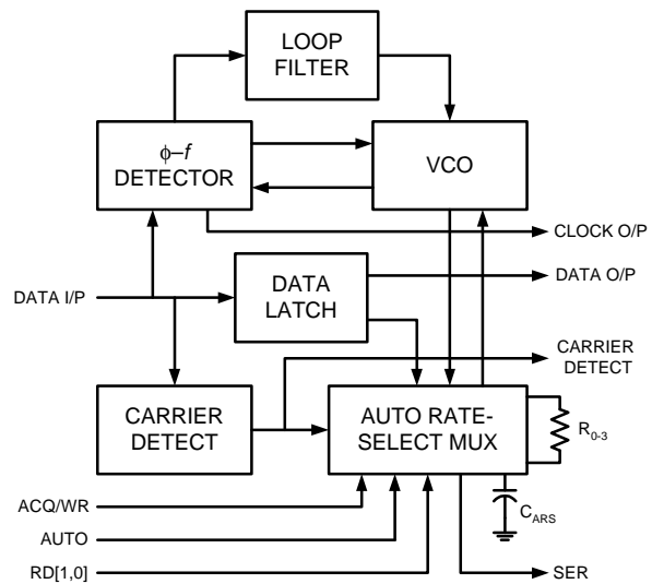
CLC016 Data Retimer/Clock Separator
