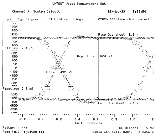
CLC016 Data Retimer Output (CLC020 source with 1m cable)
