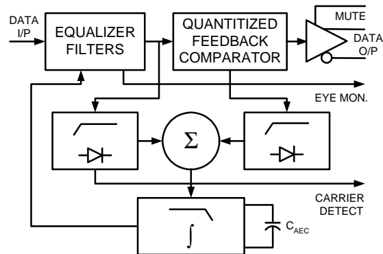
CLC014 Adaptive Cable Equalizer
