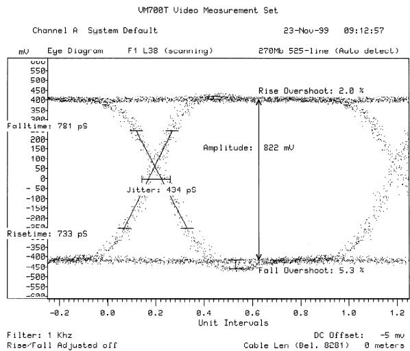
CLC016 Data Retimer Output (CLC020 source with 150m cable)
