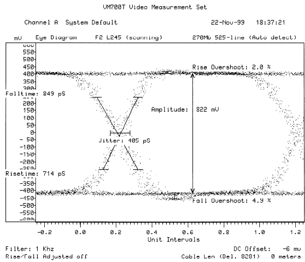
CLC014 Cable Equalizer Output (CLC020 source with 1m cable)
