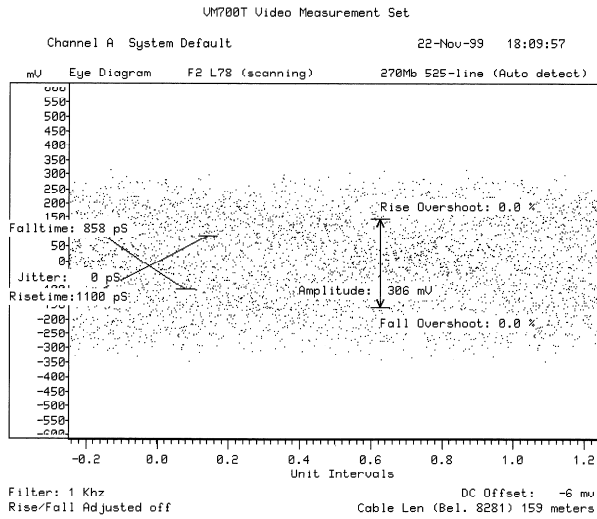
CLC020 Output after 150m of Belden 8281
