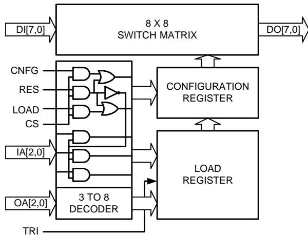
CLC018 Digital Crosspoint Switch
