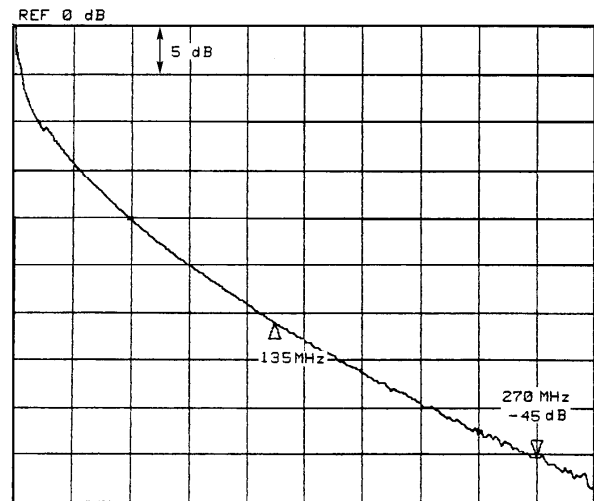
Coaxial Cable Attenuation Versus Frequency
