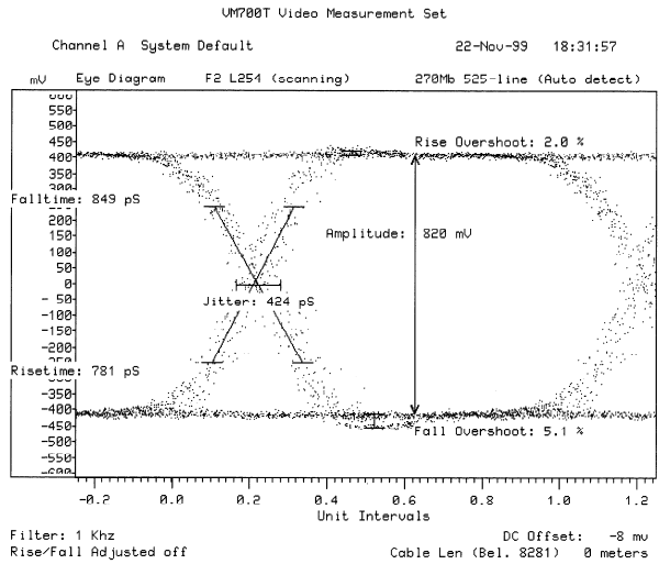
CLC014 Cable Equalizer Output (CLC020 source with 150m of Belden 8281)
