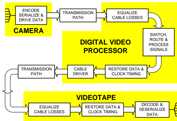
Generalized SDV Data Path
