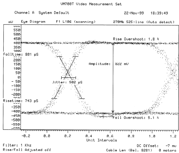
CLC016 Data Retimer Output (CLC020 source with 300m cable)
