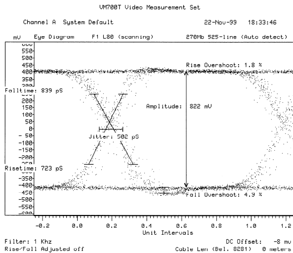
CLC014 Cable Equalizer Output (CLC020 source with 300m of Belden 8281)
