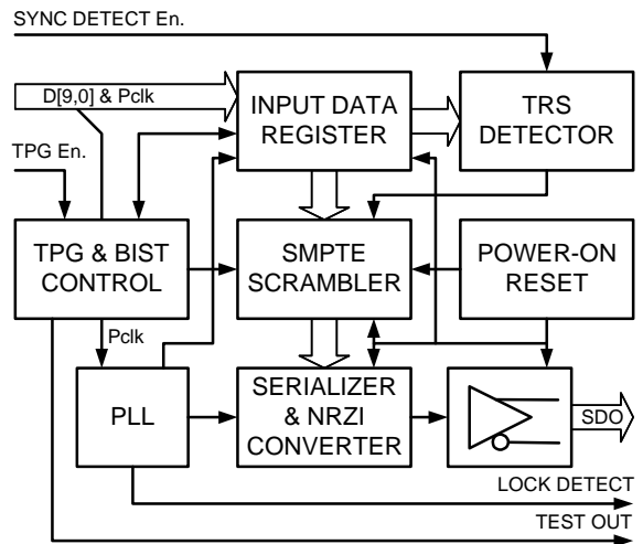
CLC020 SDV Encoder With Integral Cable Driver
