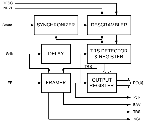
CLC011B Serial Digital Video Decoder
