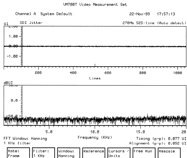
CLC020 Output Jitter (SMPTE Colour Bars)
