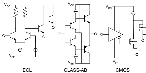
SDV Driver Output Types
