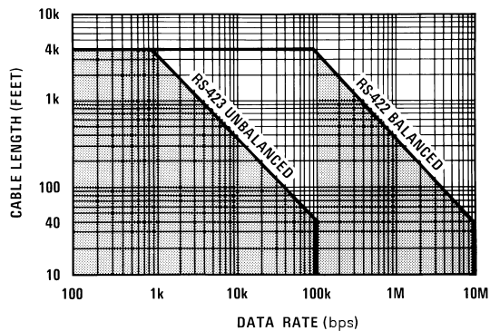
FIGURE 1. Data Modulation Rate vs Cable Length
