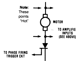
AC LINE FROM FULL WAVE BRIDGE FIGURE 2.
