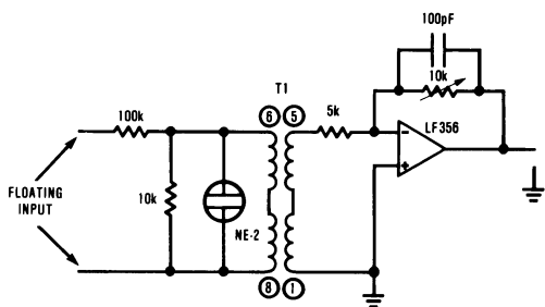
OUTPUT= INPUT \div 100 & ISOLATED T1=UTC #P2 TO AC LINE FROM FULL WAVE BRIDGE FIGURE 1.
