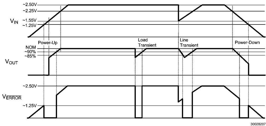
FIGURE 5. \overline{\text{ERROR}} Flag when Pull-Up is from V_{IN}
