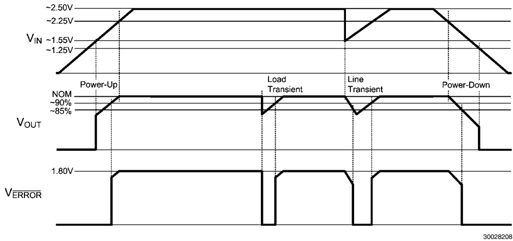
FIGURE 4. \overline{\text{ERROR}} Flag when Pull-Up is from V_{OUT}
