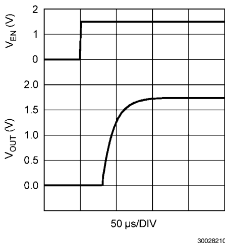
FIGURE 1. V_{OUT} vs. V_{EN}
