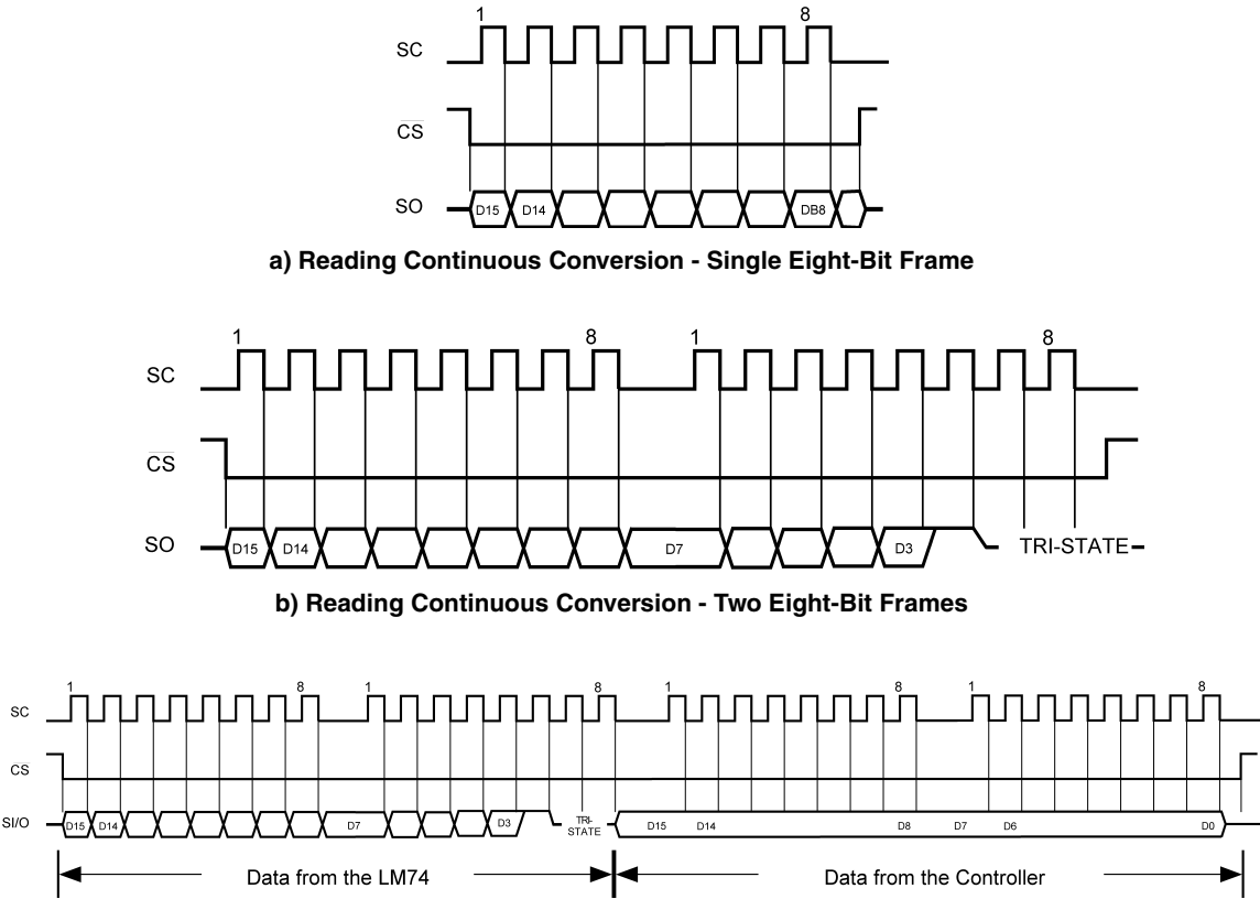
c) Writing Shutdown Control FIGURE 7. Timing Diagrams
