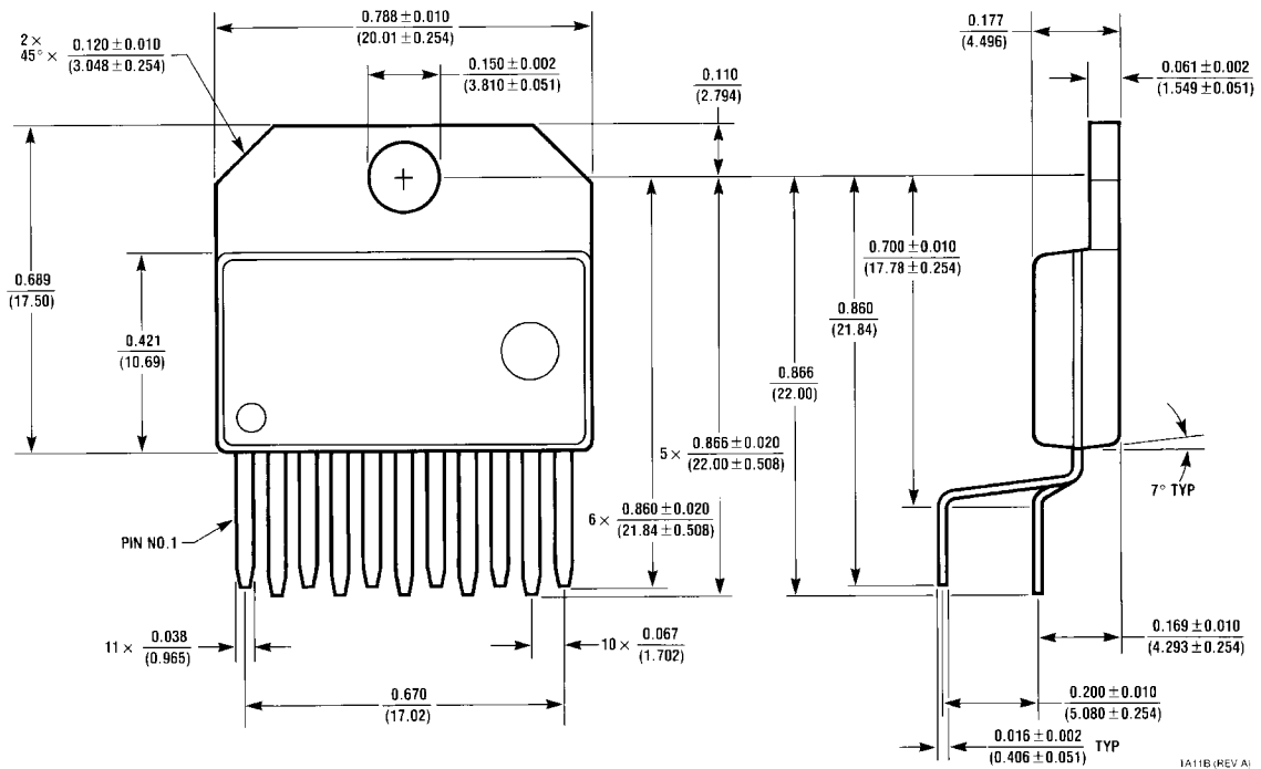
Order Number LM3876T NS Package Number TA11B
