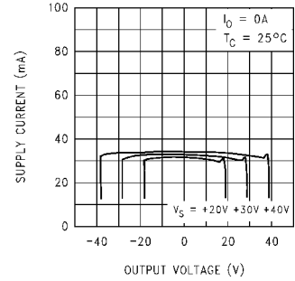
Supply Current vs Output Voltage
