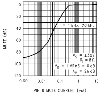
Mute Attenuation vs Mute Current
