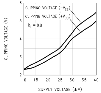
Clipping Voltage vs Supply Voltage
