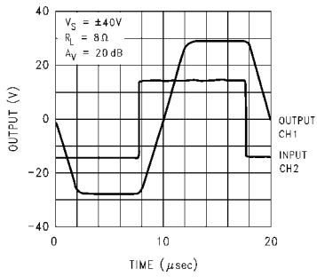
Pulse Response
