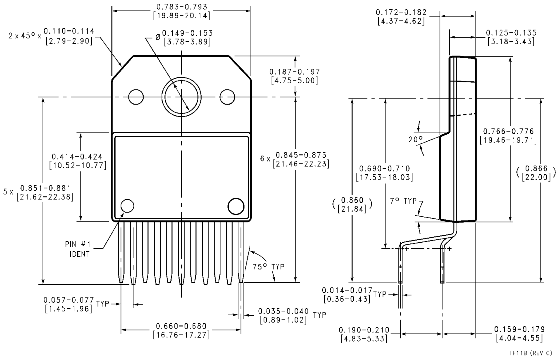
Order Number LM3876TF NS Package Number TF11B
