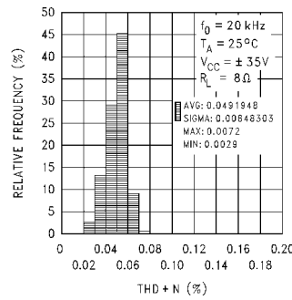
THD + N Distribution
