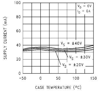
Supply Current vs Case Temperature
