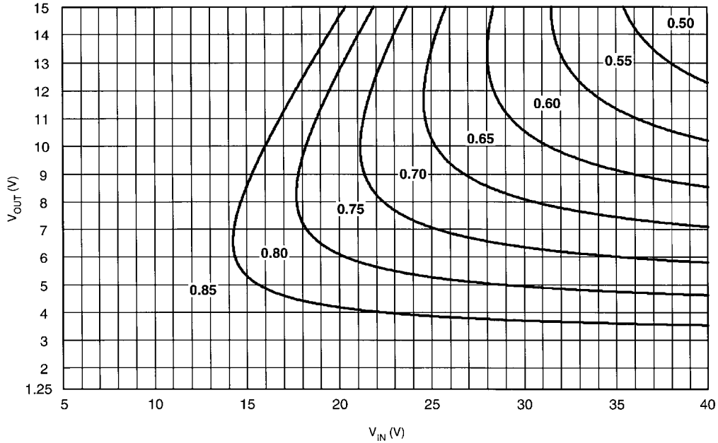
FIGURE 6. LM2825 Output Current Derating for T_J = -40 \sim -25
