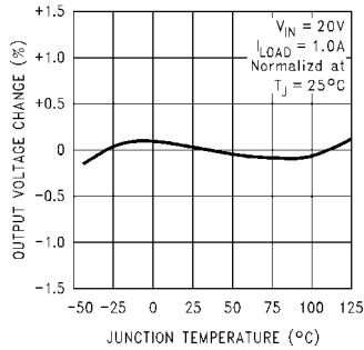
Normalized Output Voltage
