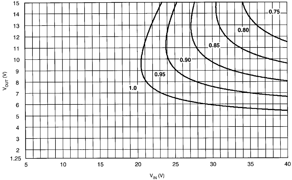
FIGURE 8. LM2825 Output Current Derating for T_A = 0 \sim 70
