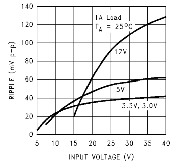
Output Ripple Voltage
