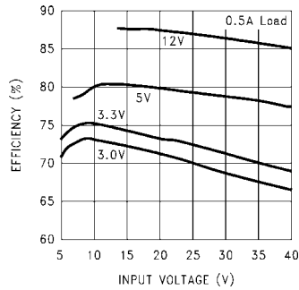
Efficiency
