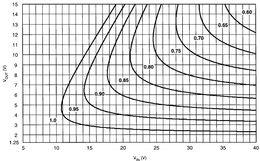
FIGURE 7. LM2825 Output Current Derating for T_J = -25 \sim 0
