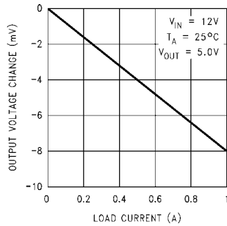
Load Regulation
