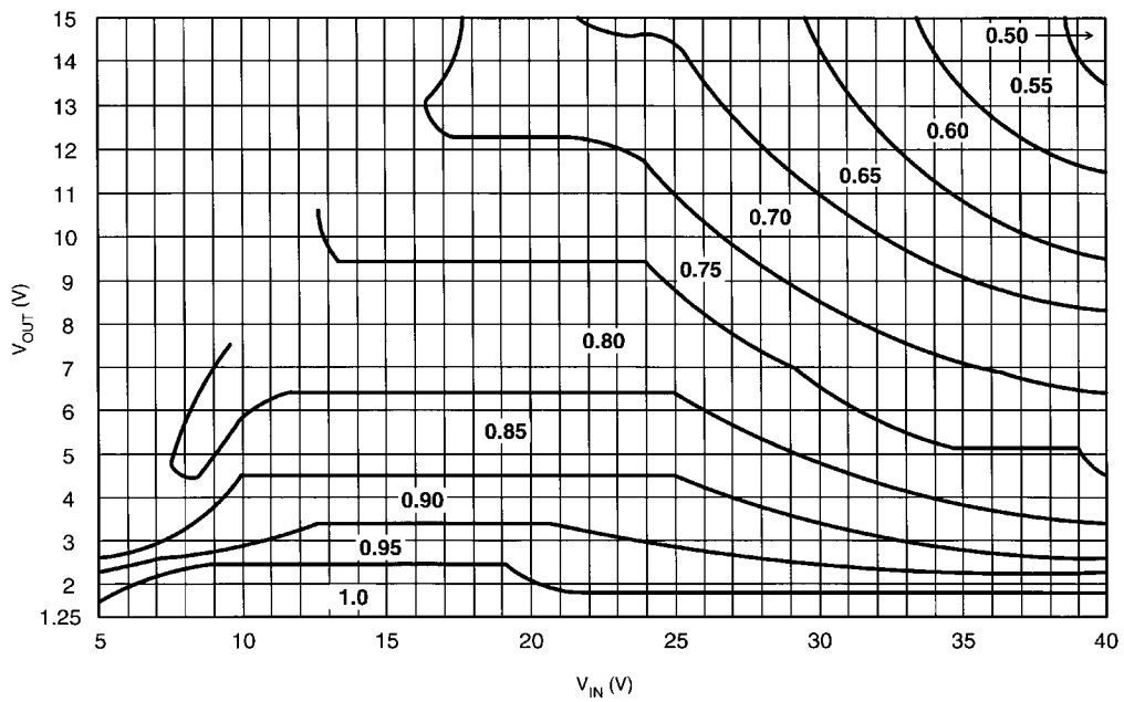
FIGURE 9. LM2825 Output Current Derating for T_A = 70 \sim 85
